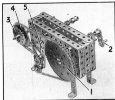
Fig. 5. A Derailleur type change-speed mechanism assembled on a demonstration framework.
