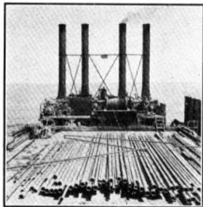
A drilling barge on Lake Maracaibo.
