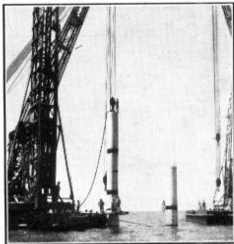
Sinking caissons in readiness for boring for oil under Lake Maracalbo.
